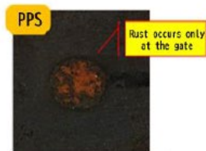
Fig. Gate part of molded product
